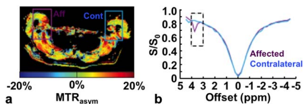
FIGURE 5: APT MRI of lymphedema. a: A spatial map and b: CEST spectra of MTR_{\text{asym}} with saturation at 1 \mu\text{T} for 75 msec at 3T magnetic field strength shows stronger CEST in the affected lymphedematous arm (Aff) than the contralateral arm (Cont) of a 42-year-old female patient previously treated for breast cancer with tamoxifen chemotherapy. Adapted with permission from Ref. 63.
