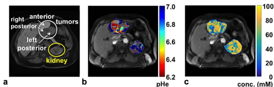
FIGURE 12: AcidoCEST MRI of cancer. a: An anatomical image of a 69-year-old patient with a high-grade serous carcinoma showed the location of three tumors that were metastases from a prior ovarian tumor. b: The parametric map of extracellular pH showed regions of the tumors that were acidic. c: The parametric map of agent concentration showed a range from 56–84 mM in the tumors and 69–80 mM in the kidney. AcidoCEST MR images were acquired with saturation applied between 3.0 and 6.9 ppm with 1.5 \mu T power for 2 sec, using a 3T MRI scanner. 120 mL of 976 mM iopamidol (Isovue) was administered to the patient. Images were analyzed with the Bloch–McConnell equations. Adapted with permission from Ref. 112.
