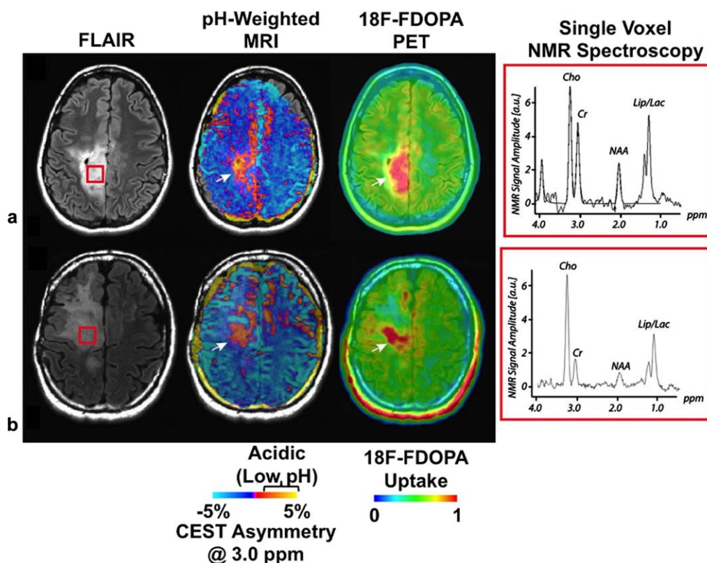
FIGURE 7: Amine CEST MRI of cancer. a,b: Two patients with anaplastic astrocytomas localized with fluid attenuated inversion recovery (FLAIR) imaging (left) showed CEST asymmetry at 3.0 ppm, which was interpreted to arise from low pH areas (center). These regions of low pH matched ^{18}\text{F} -FDOPA uptake measured with positron emission tomography (right); and c: Lactate measured from NMR spectroscopy taken from the brain area shown in the red box in the anatomical FLAIR images. Cho = choline; Cr = creatine; NAA = N-acetyl aspartate; Lip/Lac = mobile lipids and/or lactate. Adapted with permission from Ref. 81.
