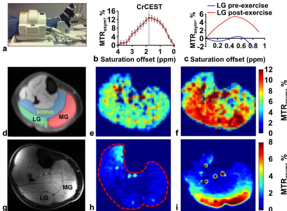
FIGURE 10: CrCEST and LATEST MRI of muscle metabolism. a: A volunteer used a foot pedal in the magnet for mild plantar flexion exercise, and the lower leg was imaged with a 28-channel knee coil. MTR_{\text{asym}} plots of b: crCEST after exercise, and c: LATEST in the later gastrocnemius muscle before and after exercise, showed strong CEST signals at 1.9 ppm and 0.5 ppm, respectively. d,g: Anatomical images of human calf muscle showed the locations of the soleus, medial gastrocnemius (MG) and lateral gastrocnemius (LG). e,h: MTR_{\text{asym}} maps before and f,i: after exercise show a signal increase the MG and LG muscles that indicated accumulation of e,f: creatine and h,i: lactic acid. CrCEST images were acquired with saturation applied at 2.9 \mu\text{T} power for 1 sec, and LATEST images were acquired with 0.73 \mu\text{T} power for 3 sec. Both image sets were corrected for B_0 and B_1 inhomogeneities. CrCEST and LATEST studies were performed at 3T and 7T magnetic field strengths, respectively. Adapted with permission from Refs. 104, 105, and 107.
