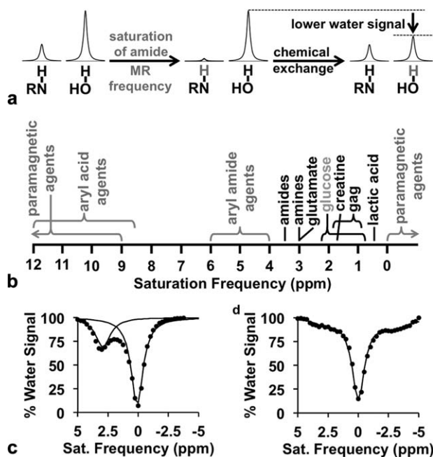
FIGURE 1: CEST MRI. a: The CEST mechanism consists of selective saturation of a labile hydrogen atom (shown in gray), and chemical exchange of this hydrogen with a hydrogen on a water molecule, which transfers the saturation to water and lowers the net coherent MR signal from water. b: Exogenous agents (gray) and endogenous biomolecules (black) are detected by applying a saturation at a specific MR frequency as listed in the chart. Many paramagnetic agents can have MR frequencies beyond the ends of the chart. c: A CEST spectrum of glutamate with 3.6 \mu\text{T} saturation power applied for 5 sec shows a decrease in % water signal at 3.0 ppm. The spectrum was fit with a sum of two Lorentzian line shapes, and each Lorentzian line shape is shown on the graph. d: An endogenous CEST spectrum of a mouse with 2 \mu\text{T} saturation power applied for 2 sec shows CEST from endogenous biomolecules at 1–3.5 ppm, and magnetization transfer from endogenous biomolecules at –2.5 to –4 ppm. The spectrum was fit with a sum of three Lorentzian line shapes, and the sum of the line shapes is shown as a solid line on the graph.
