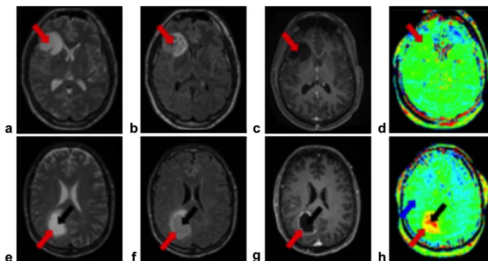
FIGURE 6: APT MRI of cancer. a–d: A 30-year-old female patient with low-grade oligodendroglioma and e–h: a 58-year-old male patient with high-grade glioblastoma were scanned. a,e: T_2 -weighted images and b,f: fluid attenuated inversion recovery images that showed the locations of the tumor rim (red arrow) and core (black arrow). c,g: Gadolinium-enhanced T_1 -weighted images showed no contrast enhancement for the low-grade tumor, and an enhancing rim with a nonenhancing central area for the high-grade tumor. d,h: APT-weighted images showed isointensity compared with contralateral brain tissue for the low-grade tumor, and hyperintensity compared to normal brain tissue (blue arrow) for the high-grade tumor. Adapted with permission from Ref. 73.
