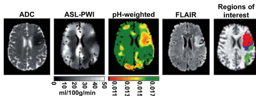
FIGURE 3: APT MRI of cerebral ischemia. A 53-year-old female patient with total anterior circulation stroke was imaged 2:48 hours after onset with diffusion-weighted MRI to obtain a map of apparent diffusion coefficient (ADC), arterial spin labeling-perfusion weighted imaging (ASL-PWI) to generate a map of cerebral blood flow, and APT MRI with saturation at 0.55 \mu\text{T} for 2 sec at 3T to generate a pH-weighted map (scale in arbitrary units). The patient was imaged 34 days later with fluid attenuated inversion recovery (FLAIR) MRI, and regions of interest were identified (green = oligemia; blue = infarct growth; red = ischemic core). Adapted with permission from Ref. 57.
