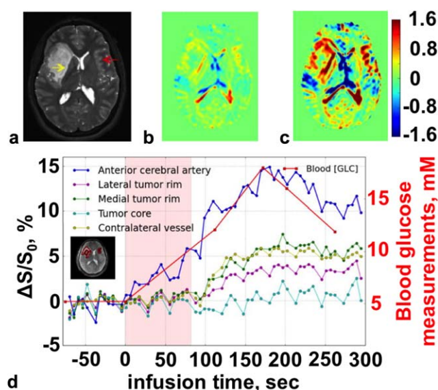
FIGURE 11: GlucoCEST MRI of cancer. a: An anatomical T_2 -weighted MR image showed the location of the tumor (yellow arrow). b: The increase in CEST signal after saturation was applied at 1.96 \mu\text{T} power for 2.4 sec at 1.2 ppm between 0 and 110 sec after starting the infusion, and c: between 110 and 295 sec after starting the infusion, showed the glucose accumulation in the tumor rim. d: The dynamic changes in \text{MTR}_{\text{asym}} signal showed the rate of glucose uptake in various tumor regions. Adapted with permission from Ref. 115.
