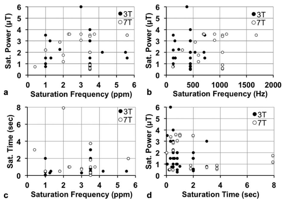
FIGURE 2: Clinical CEST MRI saturation parameters. A total of 60 published reports were surveyed that listed saturation power, time, magnetic field strength, and single saturation frequency that was analyzed. a,b: The saturation powers used in clinical CEST MRI studies have not been correlated with the investigated saturation frequencies, in units of ppm or Hz (ppm \times magnetic field strength). c: The saturation times used in clinical CEST MRI studies have not been correlated with saturation frequency. d: The saturation powers and times used in clinical CEST MRI studies have not been correlated. An additional 10 studies that analyzed a range of saturation frequencies were not included in these graphs. Yet these 10 additional studies also did not show correlations between saturation parameters.
