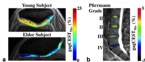
FIGURE 8: GagCEST MRI of knee and spine. a: Maps of patellar cartilage in a young volunteer and an elderly 65-year-old male patient with knee pain showed differences in gagCEST signal, after applying 2.2 \mu\text{T} saturation for 0.5 sec at 7T magnetic field strength. b: GagCEST signal at 0.5–1.5 ppm was measured with 0.8 \mu\text{T} saturation power applied for 1 sec at 3T magnetic field strength, which was overlaid on a sagittal T 2 -weighted MR image of lumbar intervertebral disks of a 41-year-old male patient. Decreased gagCEST contrast was observed with increasing Pfirrmann grade that scores intervertebral disk degeneration. Adapted with permission from Refs. 97 and 99.
