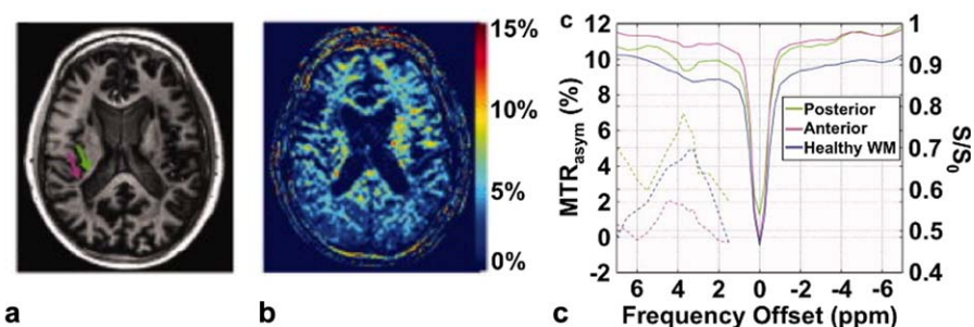
FIGURE 4: APT MRI of multiple sclerosis. a: A T_1 -weighted MR image identified the heterogeneous periventricular lesion with an anterior hypointense region (green arrow) and a posterior hyperintense region (magenta arrow). b: The MTR_{\text{asym}} map with saturation at 3.5 \mu\text{T} for 1 sec at 7T magnetic field strength showed that the lesion had increased MTR_{\text{asym}} . c: CEST spectra (right y-axis) and MTR_{\text{asym}} (left y-axis) showed strongest CEST signal in the posterior region. Adapted with permission from Ref. 60.
