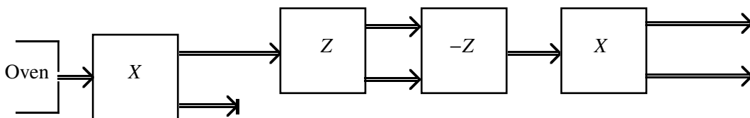
Figure 6.9: Atomic beam for which S_x = \frac{1}{2} \hbar split into S_z = \pm \frac{1}{2} \hbar beams and then recombined before passing through a final Stern-Gerlach device with magnetic field in x direction.
